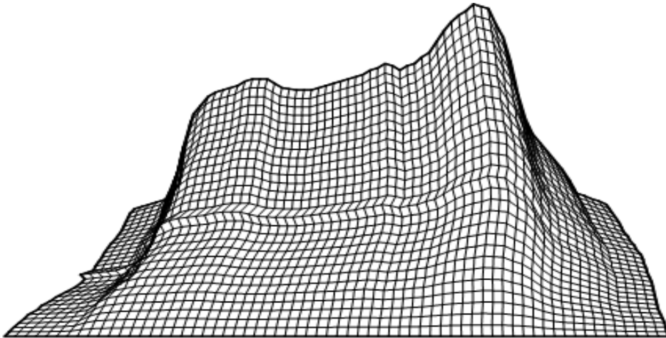
Figure 3a. Curvilinear boundaries and the curvilinear grid system.
