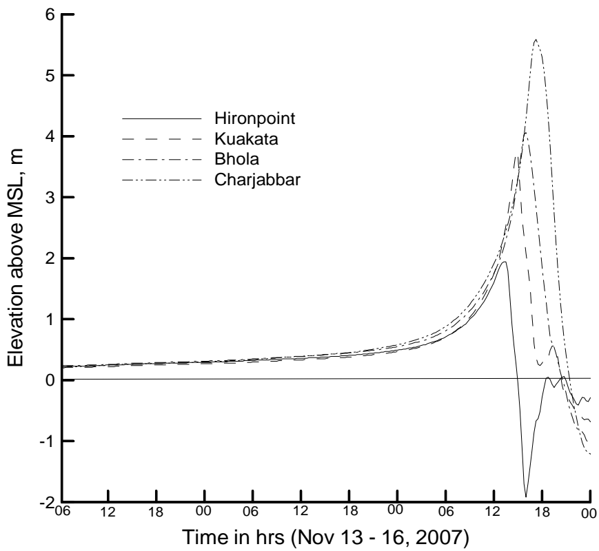
Figure 4a. Computed time series of surge levels at the coastal locations associated with November 2007 storm (Sidr).
