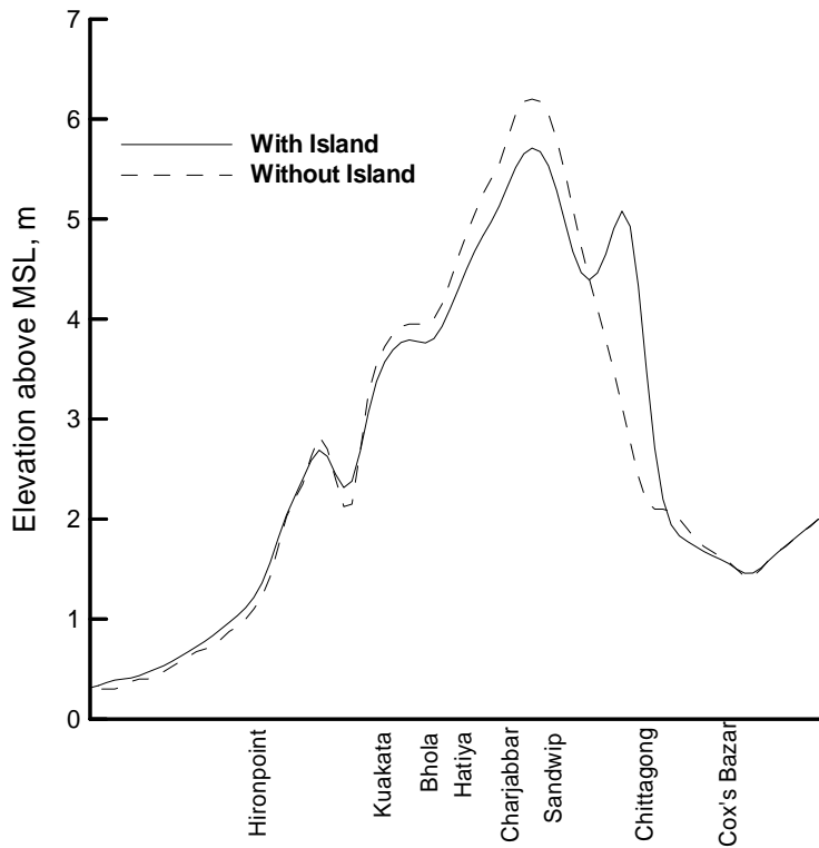
Figure 9. Maximum surge levels at different coastal locations due to 2007 storm in the presence of island and in the absence of island.
