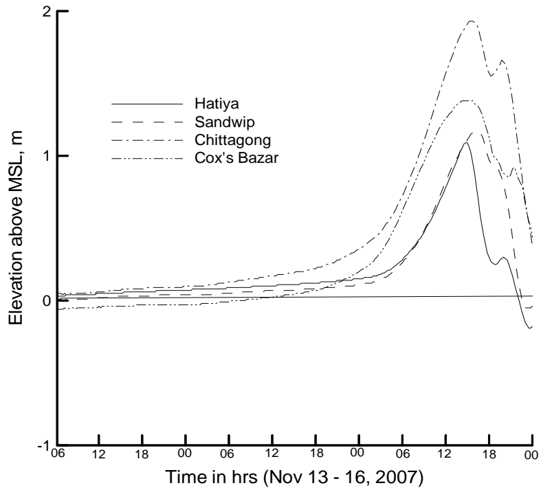
Figure 4b. Computed time series of surge levels at the coastal locations associated with November 2007 storm (Sidr).
