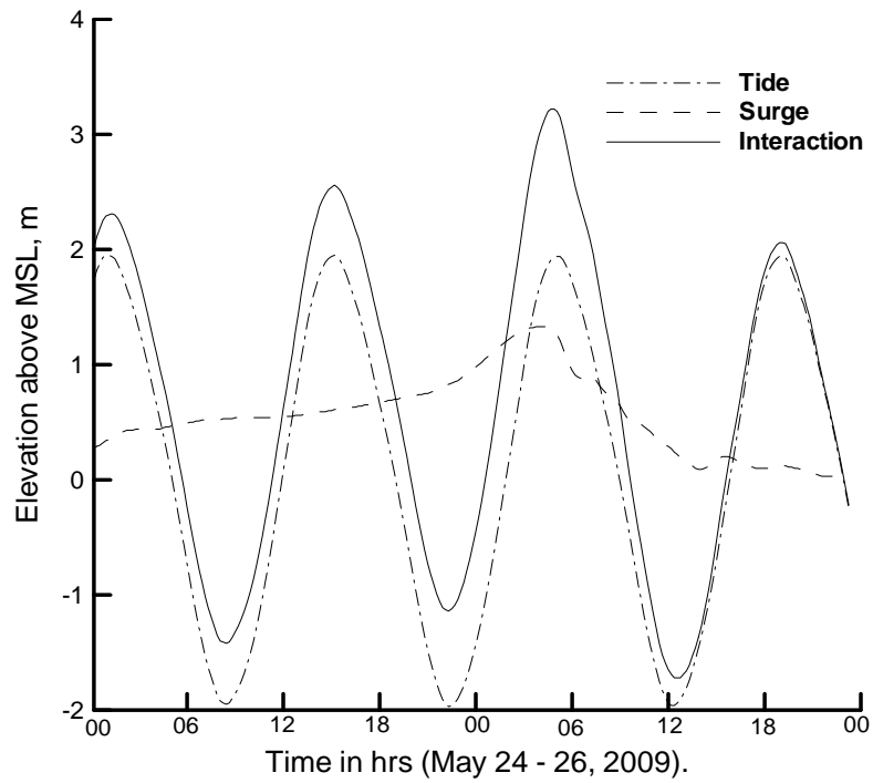
Figure 8b. Computed tide, computed surge, and their linear interaction associated with May 2009 storm at Kuakata.
