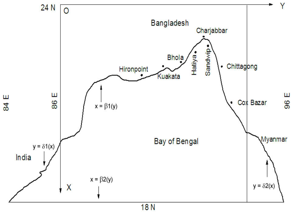
Figure 2. Boundaries of the analysis area and the locations.
