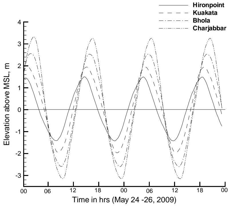
Figure 7a. Computed tidal oscillations at different coastal locations.
