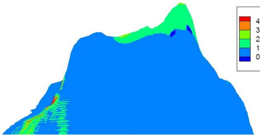
Fig 10b. Contours (in meters) of equal sea surface elevation for peak surge (without tidal consideration) along the Bay of Bengal for the storm Aila (2009).
