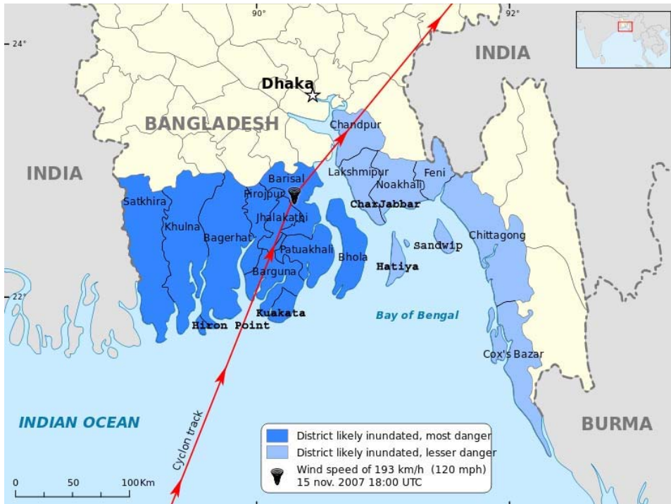
Figure 1a. Path of Cyclone Sidr (2007) and affected area with the analysis and the locations at which results are presented. Source: Bangladesh Space Research and Remote Sensing Organization.
