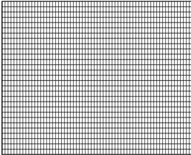
Figure 3b. Boundaries and rectangular grid system in the transformed domain.
