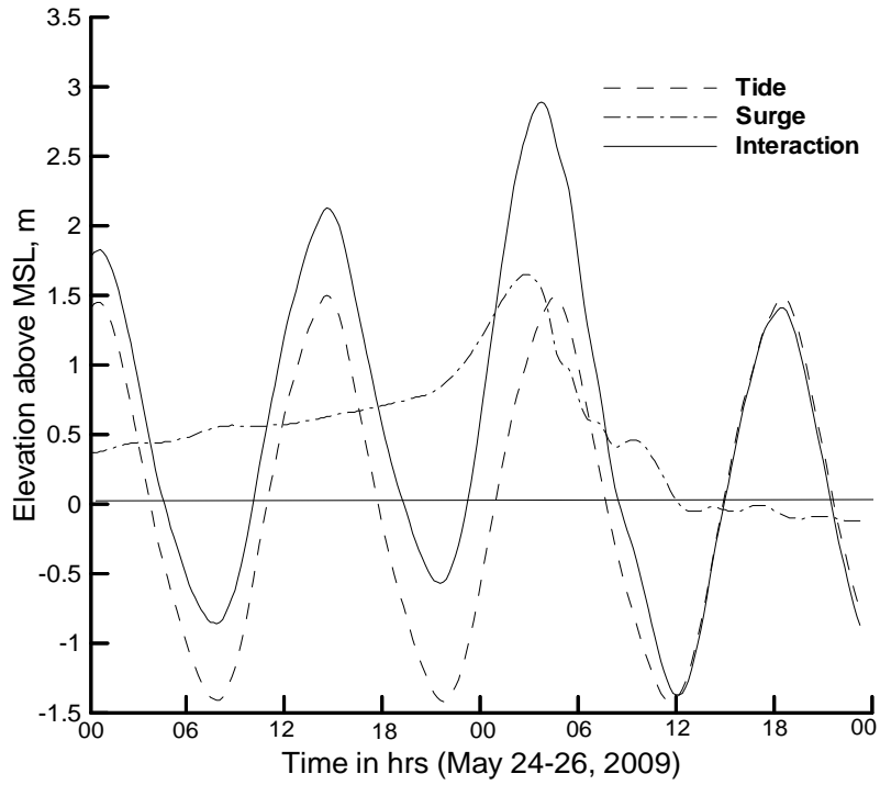
Figure 8a. Computed tide, computed surge, and their linear interaction associated with May 2009 storm at Hiron Point.
