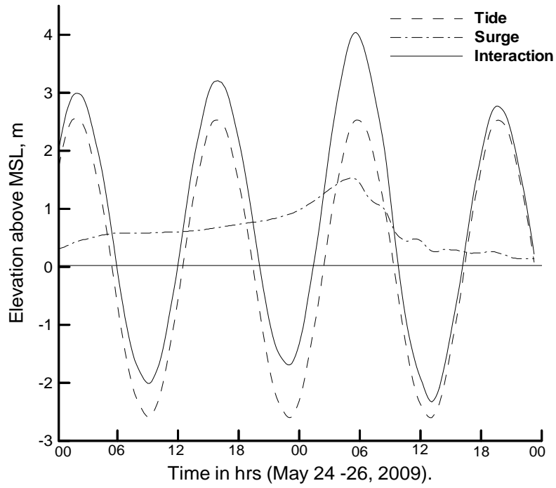
Figure 8c. Computed tide, computed surge, and their linear interaction associated with May 2009 storm at Bhola.
