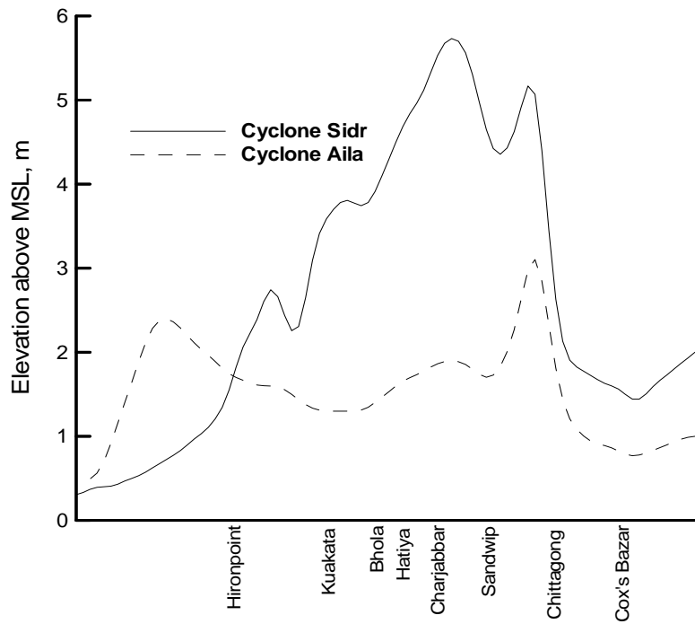
Figure 6. Peak surges along the coastal locations due to the storms of 2007 (Sidr) and 2009 (Aila).
