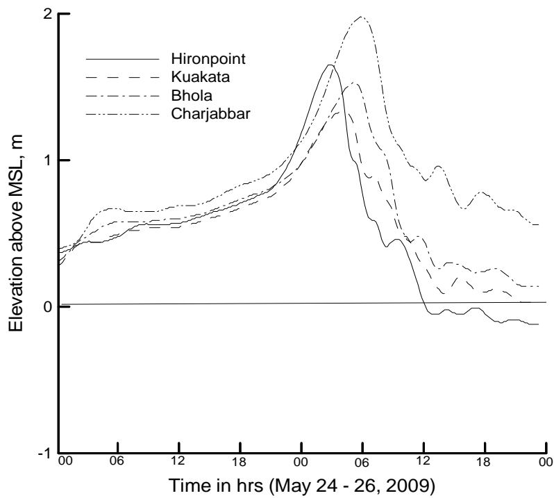
Figure 5a. Computed time series of surge levels at the coastal locations associated with May 2009 storm (Aila).
