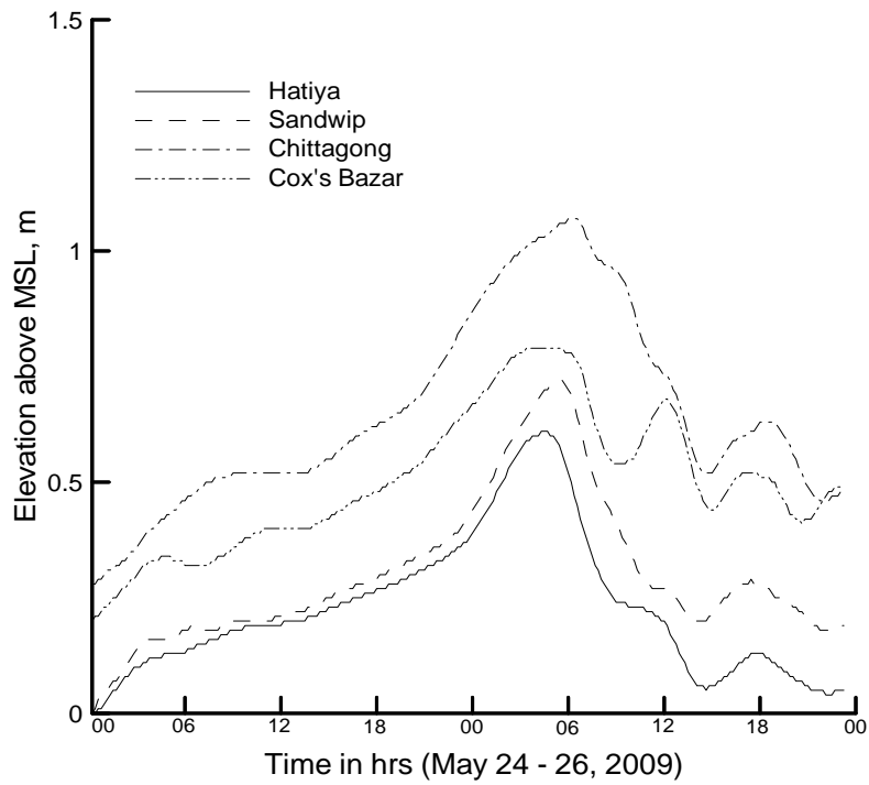
Figure 5b. Computed time series of surge levels at the coastal locations associated with May 2009 storm (Aila).
