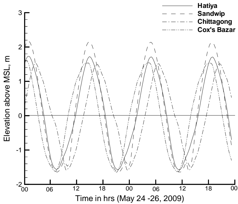
Figure 7b. Computed tidal oscillations at different coastal locations.
