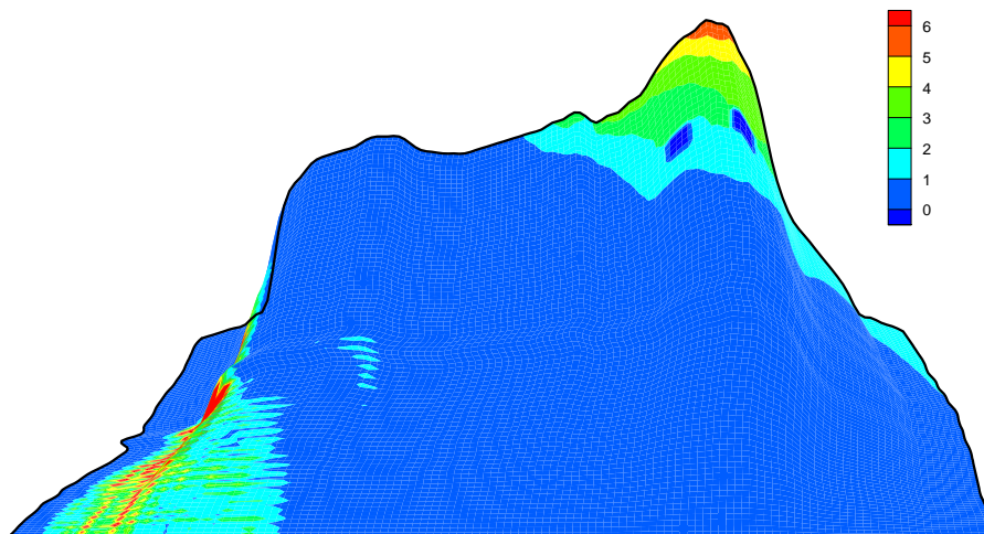
Fig 10a. Contours (in meters) of equal sea surface elevation for peak surge along the Bay of Bengal for the storm Sidr(2007).
