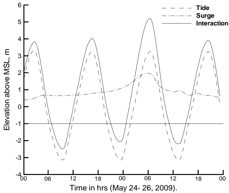
Figure 8d. Computed tide, computed surge, and their linear interaction associated with May 2009 storm at Charjabbar.
